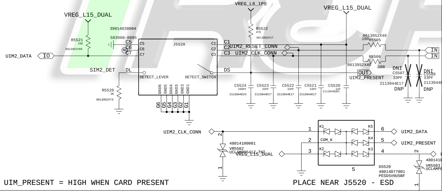
UIM2 REF:5520-5529
